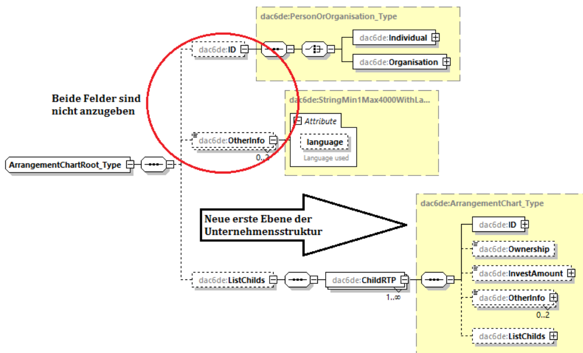
Figure 2: ArrangementChartRoot_Type with more than one top element
