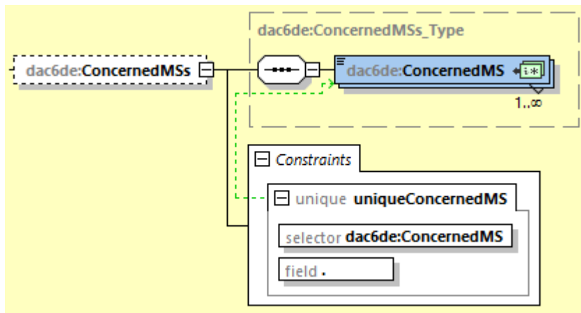
Figure 4: XML structure unique constraint
